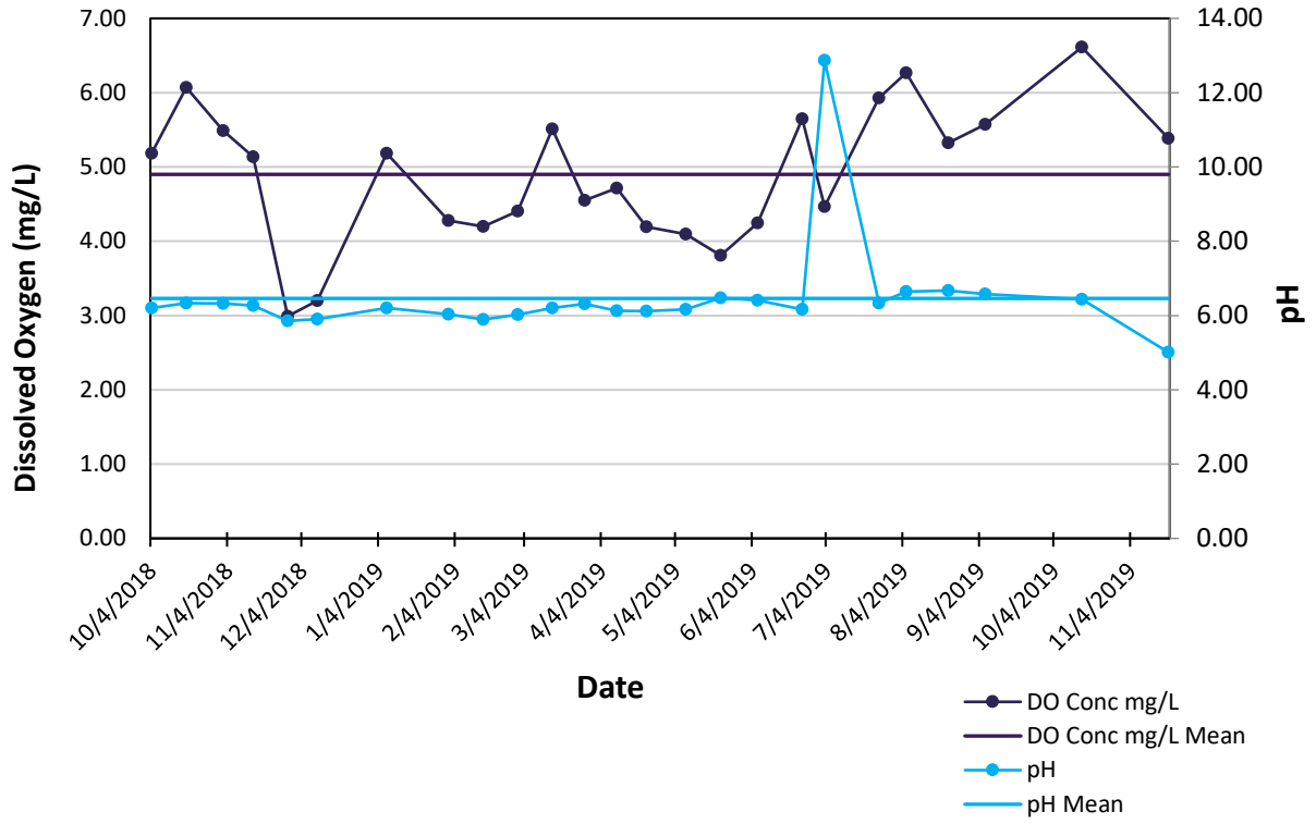
Reservation Wetland Well 1 Average Dissolved Oxygen & pH
